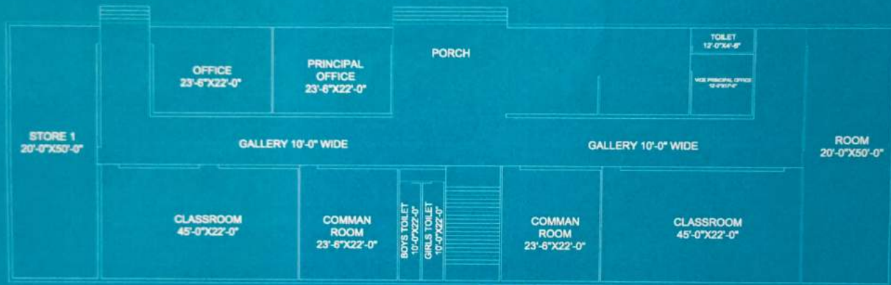
GROUND FLOOR
